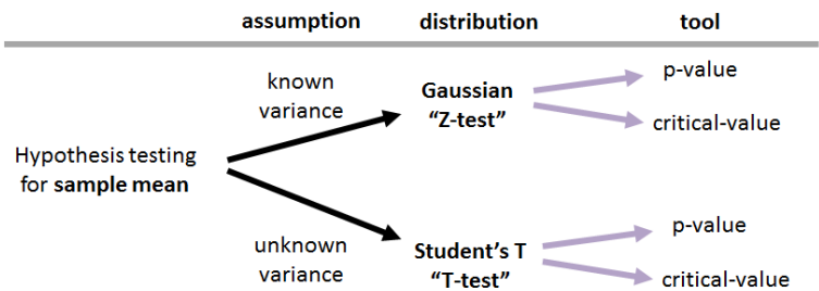
Figure 9.14: When conducting a hypothesis testing of the sample average, we may or may not know the variance. If we know the variance, we use the Gaussian distribution to conduct either a p -value test or a critical-value test. If we do not know the variance, we use Student's t -distribution.
