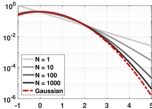
Figure 6.22: CLT fails at the tails. We note that X_1, \dots, X_N are i.i.d. exponential with a parameter \lambda = 1 . We plot the PDFs of the normalized sample average Z_N = \frac{\bar{X}_N - \mu}{\sigma/\sqrt{N}} by varying N . We plot the PDF of the standard Gaussian Z \sim \text{Gaussian}(0, 1) on the same grid. Note that the Gaussian approximation is good for values that are close to the mean. For the tails, the Gaussian approximation is not very accurate.
