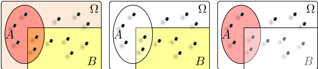
Figure 2.27: Visualization of Example 2.45: [Left] All the sets. [Middle] P(A|B) is the ratio between dots inside the light yellow region over those in yellow, which is \frac{2}{6} . [Right] P[B|A] is the ratio between dots inside the light pink region over those in pink, which is \frac{2}{5} .
