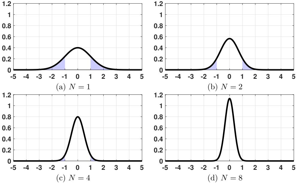
Figure 8.13: The four subfigures here illustrate the probability of error \mathbb{P}[|\hat{\Theta}_N - \theta| \geq \epsilon] , which is represented by the areas shaded in blue. We assume that the estimator \hat{\Theta}_N is a Gaussian random variable following a distribution \text{Gaussian}(0, \frac{\sigma^2}{N}) , where we set \sigma = 1 . The threshold we use in this figure is \epsilon = 1 . As N grows, we see that the probability of error diminishes. If the probability of error goes to zero, we say that the estimator is consistent .
