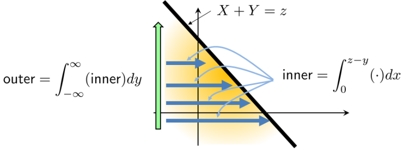
Figure 5.13: The shaded region highlights the set X + Y \leq Z . To integrate the PDF over this region, we first take the inner integration over dx and then take the outer integration over dy .
