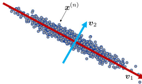
Figure 5.22: PCA aims at finding a low-dimensional representation of a high-dimensional dataset. In this figure, the 2D data points can be well represented by the 1D space spanned by \mathbf{v}_1 .
