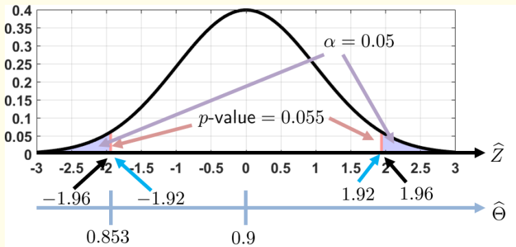
Figure 9.13: Example of a two-sided test using the p -value and the z_{\alpha} -value.
